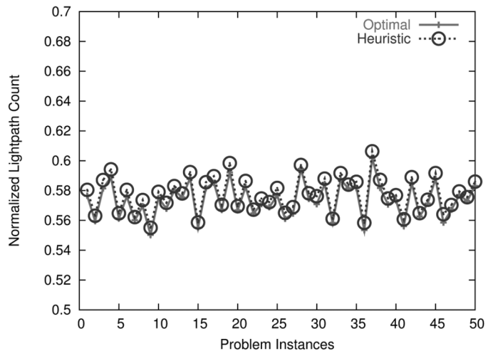
Fig. 3. Grooming effectiveness of the StarTopology algorithm, N = 10 .
