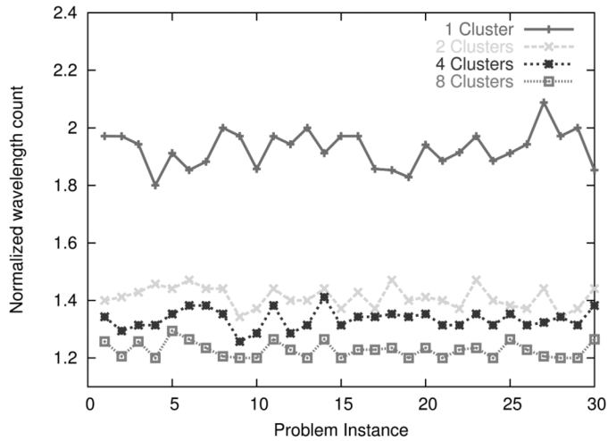
Fig. 8. Wavelength comparison, falling pattern, 32-node network.
