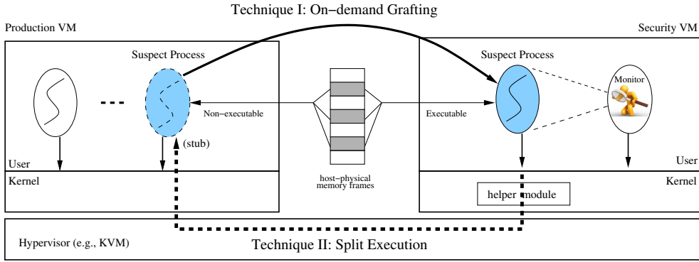
Figure 1: An Overview of Process Out-Grafting
